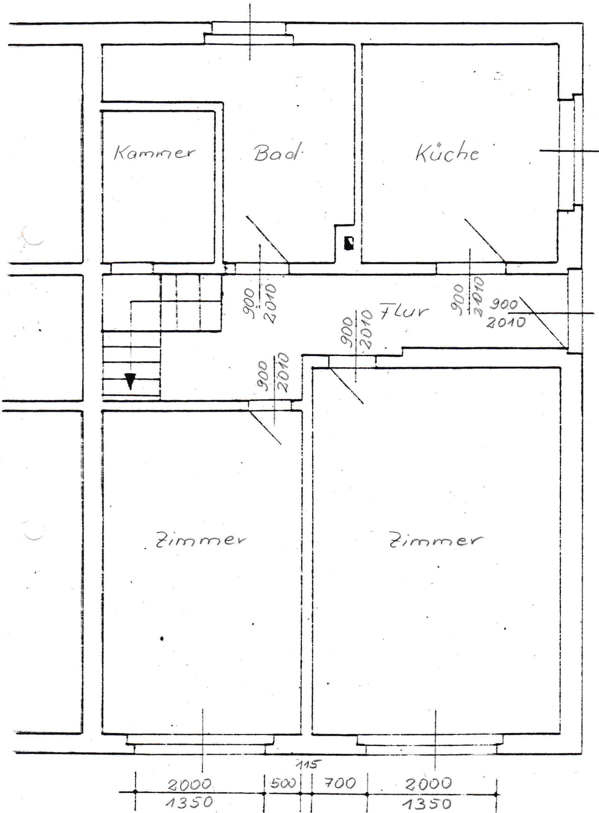
Grundriß - Erdgeschoß
