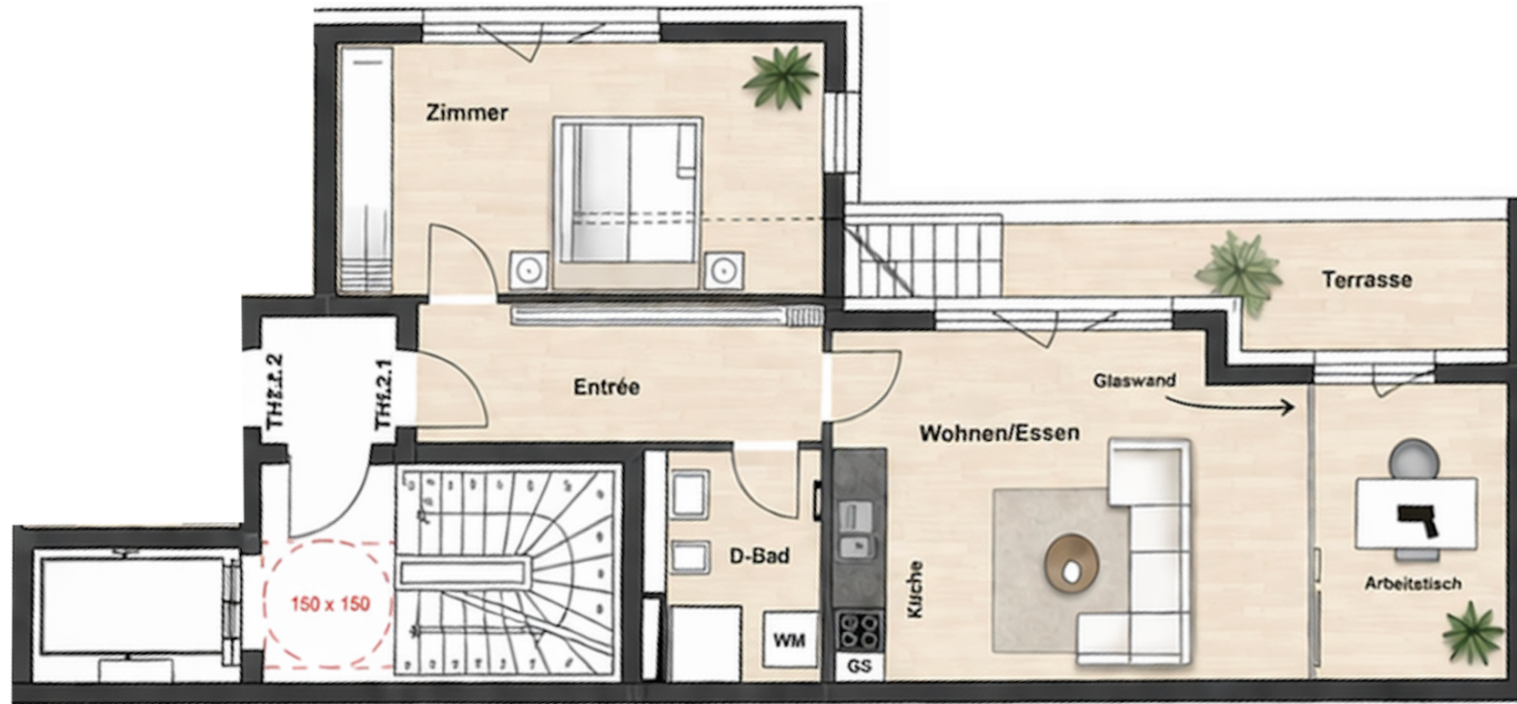
GRUNDRISS PENTHOUSE
