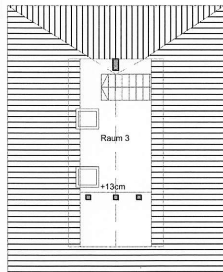
Grundriss Studio
