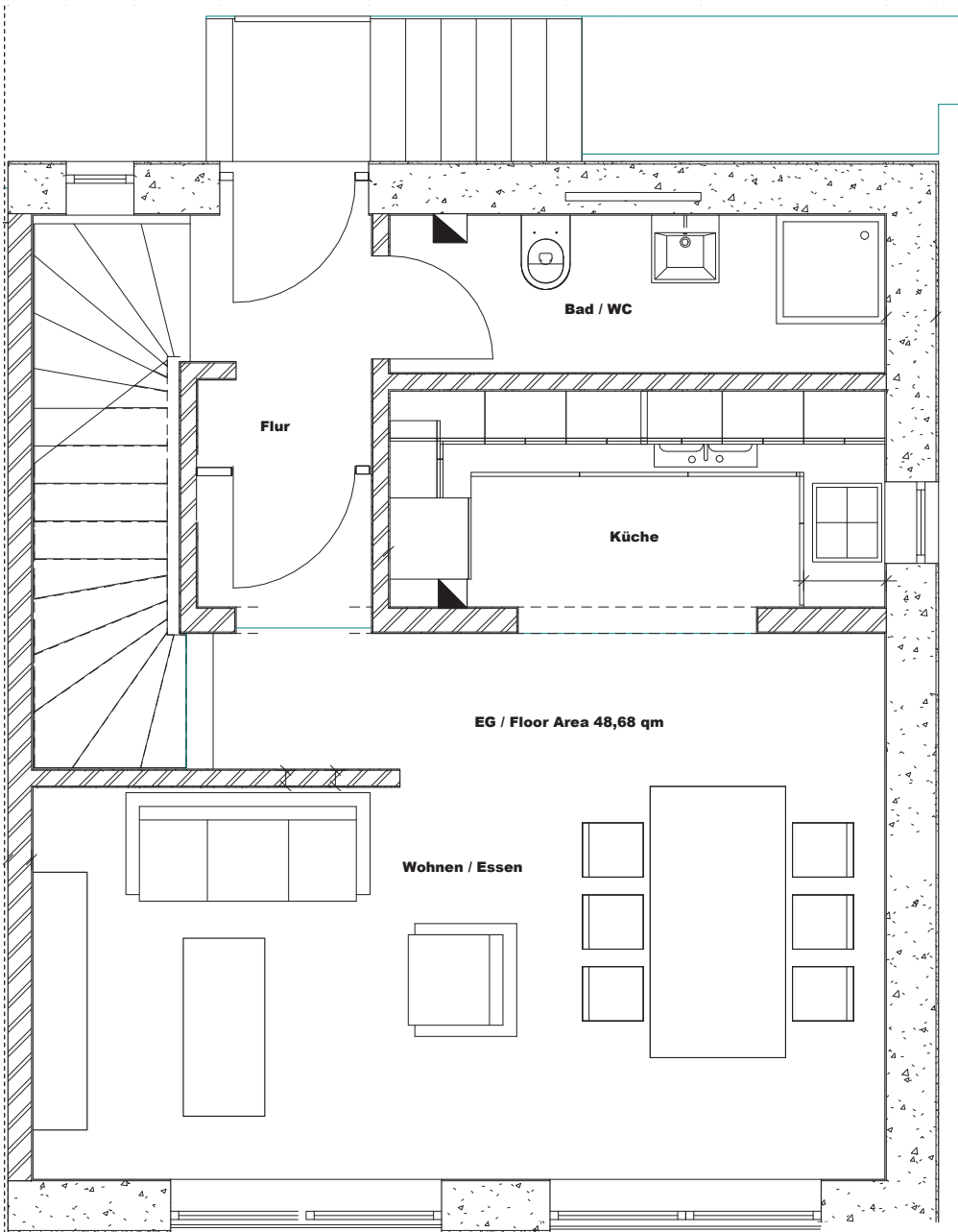
ERDGESCHOß LAYOUT
