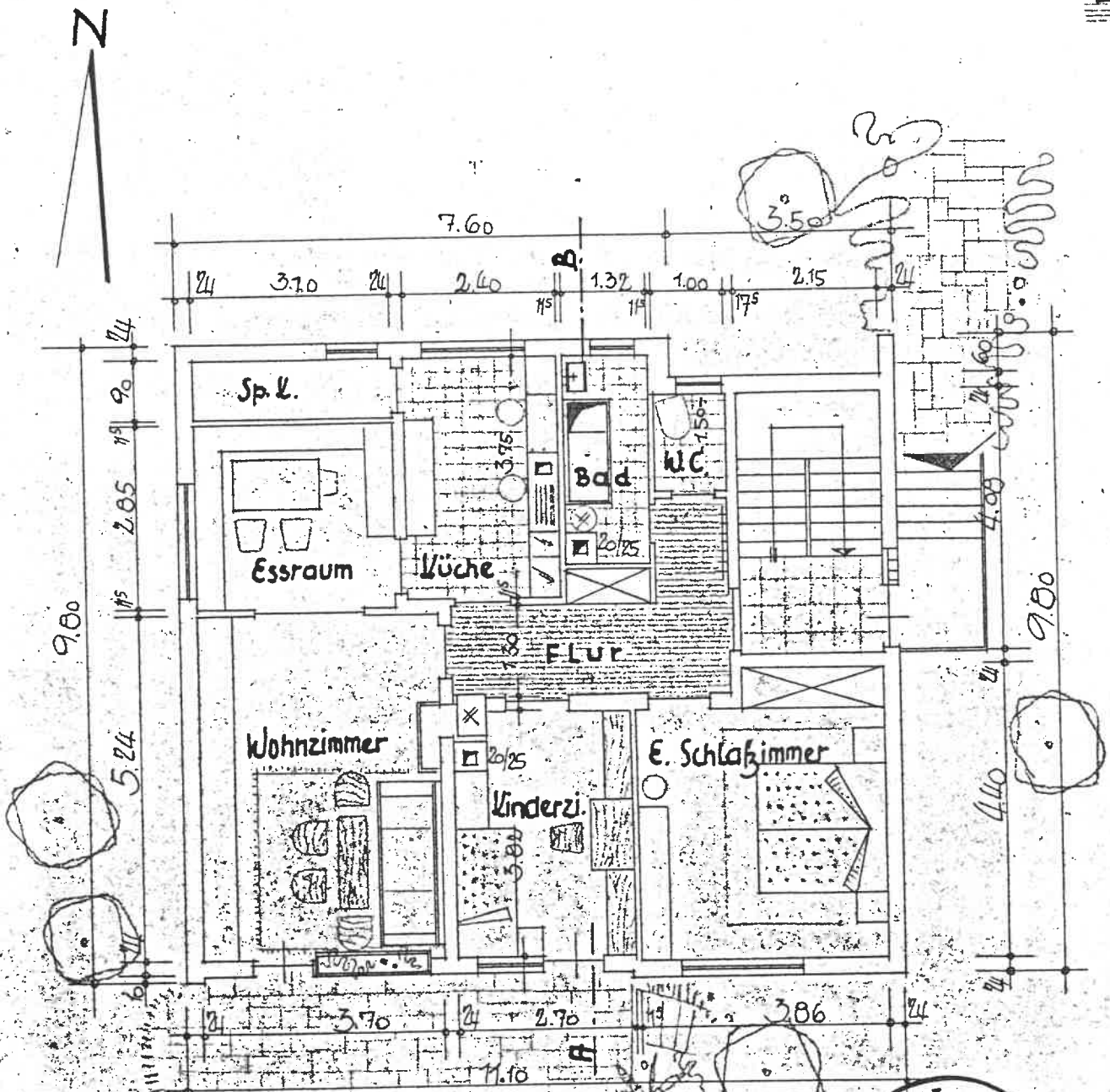
Grundriss "Erdgeschoss" 1.100
