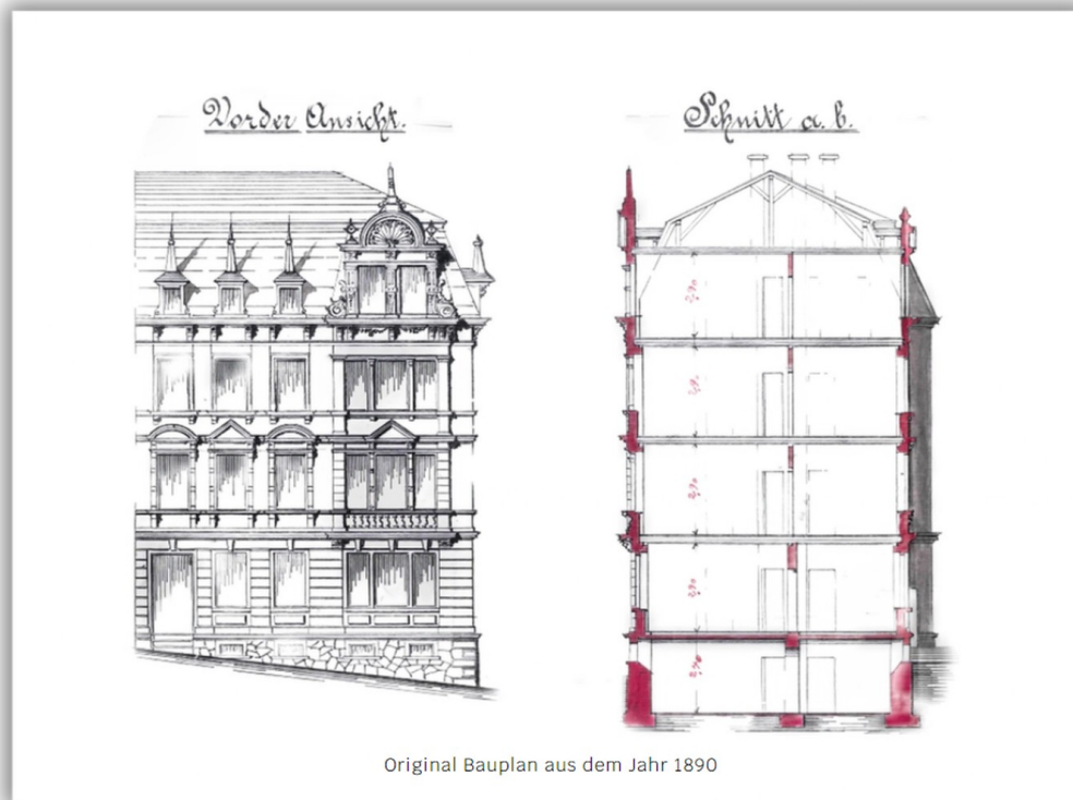
Bauplan 1890
