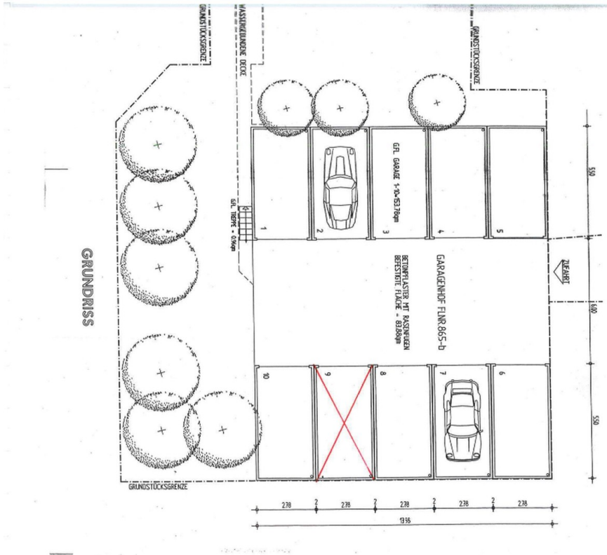
Grundriss Garage
