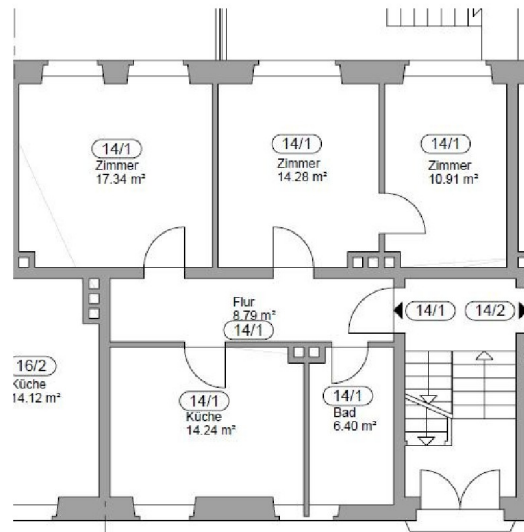
Haus Nr. 14 EG links WHG 14/1
