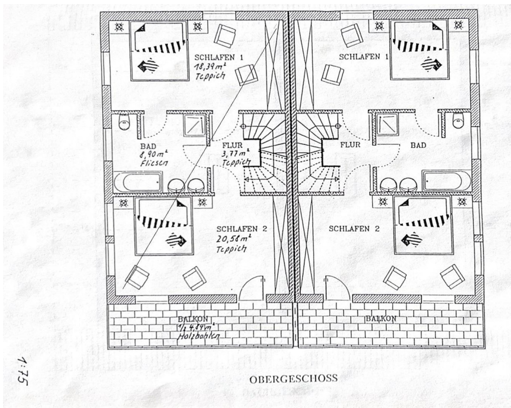
1. Stock
