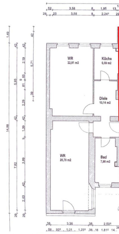
Grundriss WE 18
