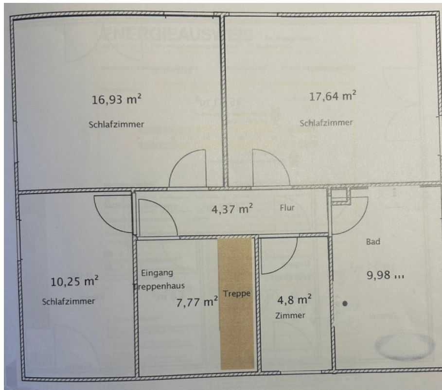
1. Stock
