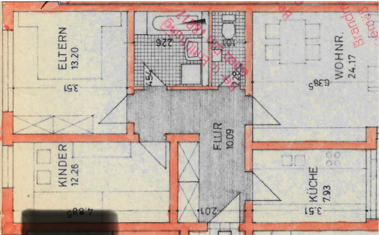
Floor Plan
