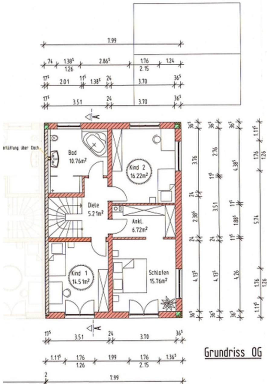
Grundriss (OG)
