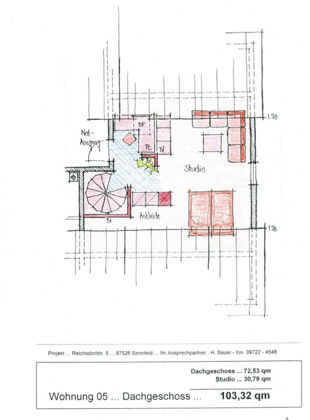
Grundriss Studio
