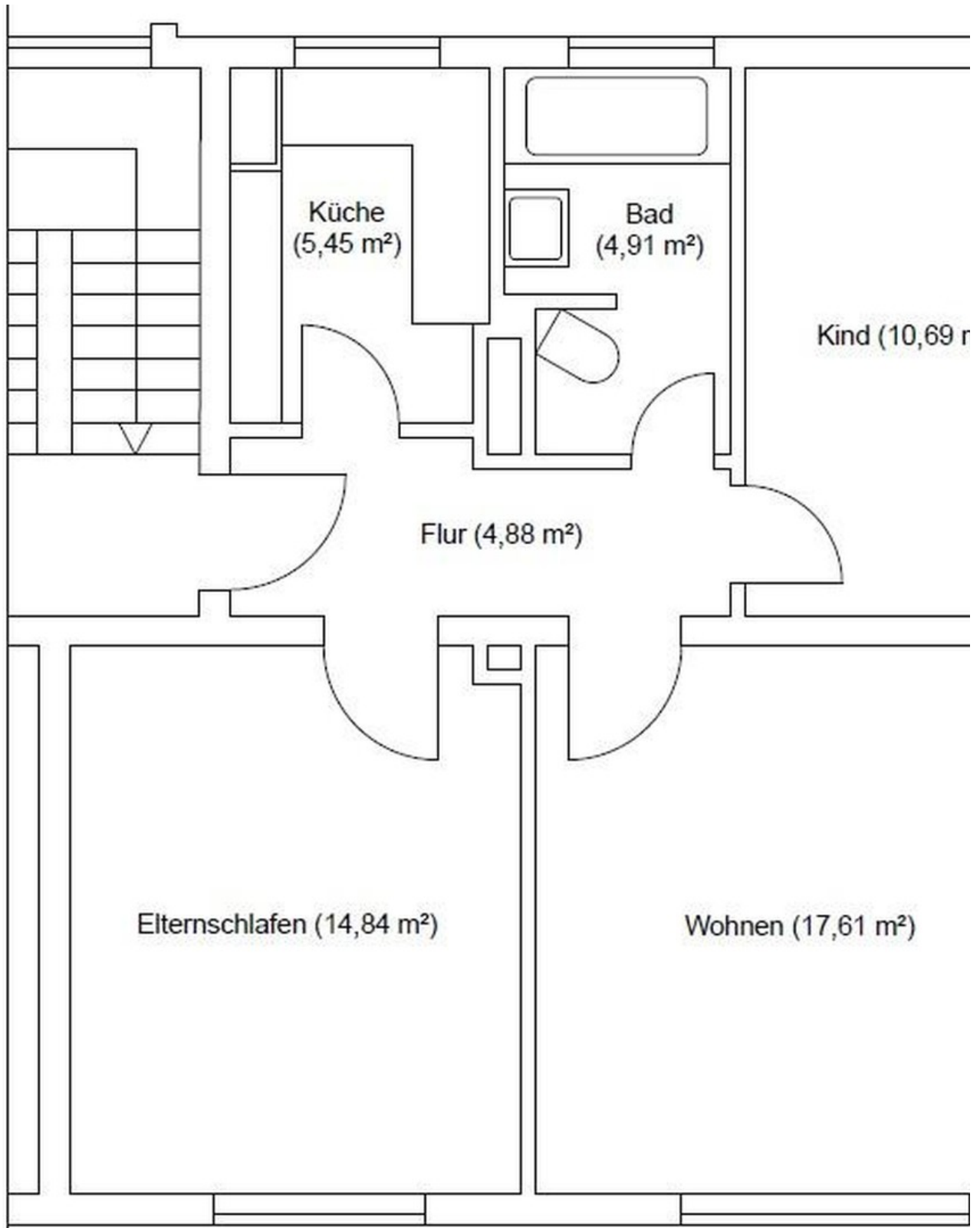
Grundriss links
