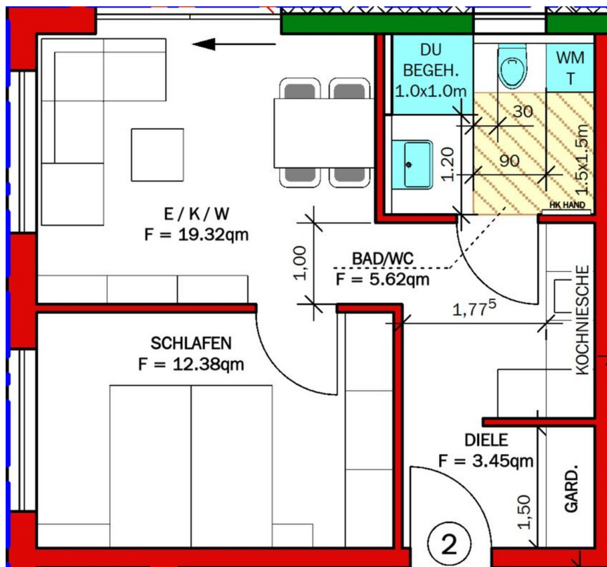
Grundriss EG links
